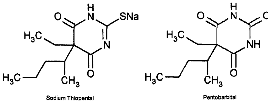
Fig. 1. The chemical structure of two barbiturates used in the lethal injection process: sodium thiopental (a barbiturate no longer available), and pentobarbital (the current substitute barbiturate).
